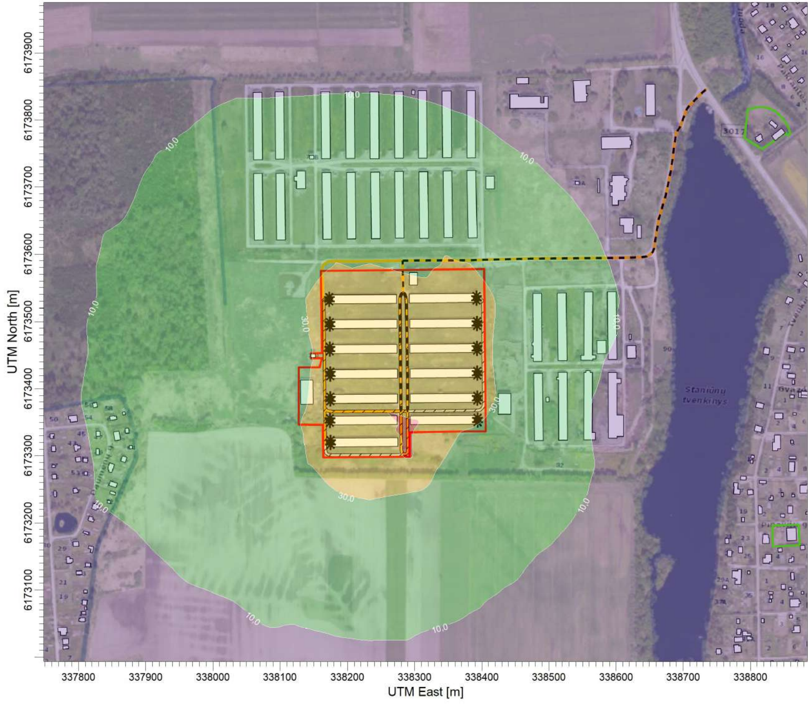
PLOT FILE OF 99.80TH PERCENTILE 1-HR VALUES FOR SOURCE GROUP: PUV Max: 52,5 [ug/m^3] at (338292,69, 6173299,34)
