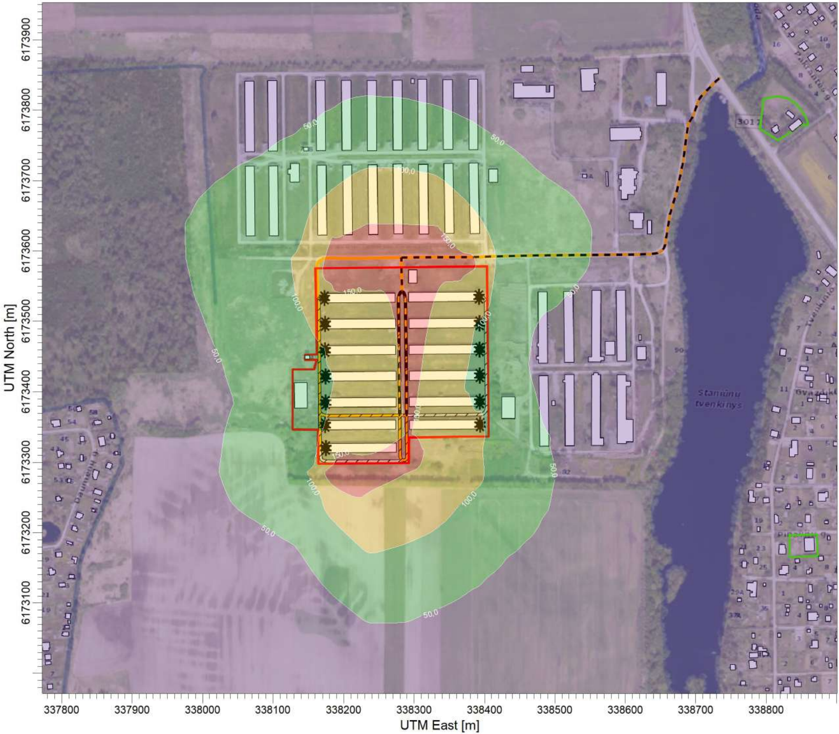
ug/m^3 PLOT FILE OF 98.50TH PERCENTILE 1-HR VALUES FOR SOURCE GROUP: ALL Max: 187,8 [ug/m^3] at (338209,06, 6173576,14)
