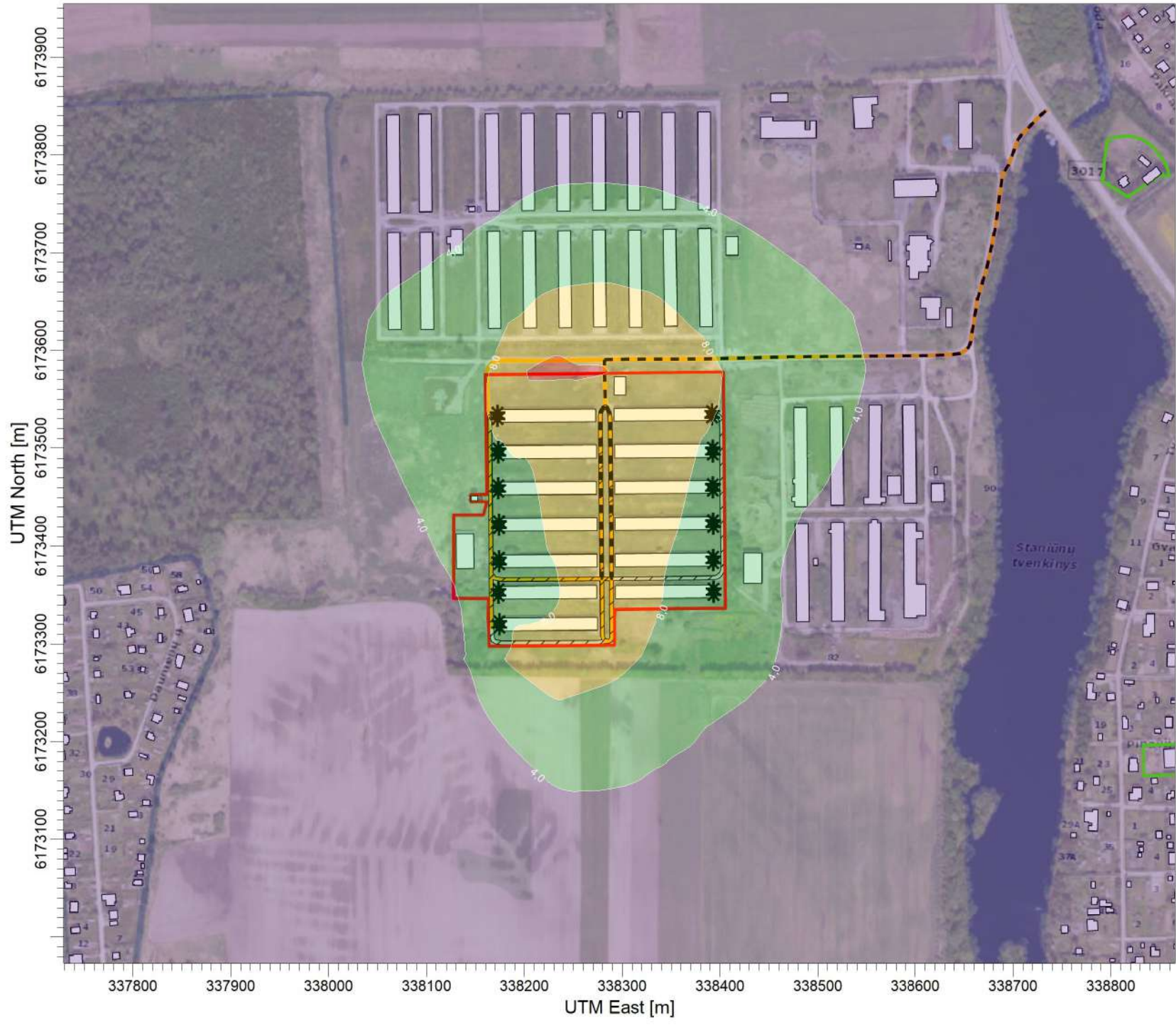
ug/m^3 PLOT FILE OF 90.40TH PERCENTILE 24-HR VALUES FOR SOURCE GROUP: PUV Max: 12,7 [ug/m^3] at (338233,03, 6173585,10)
