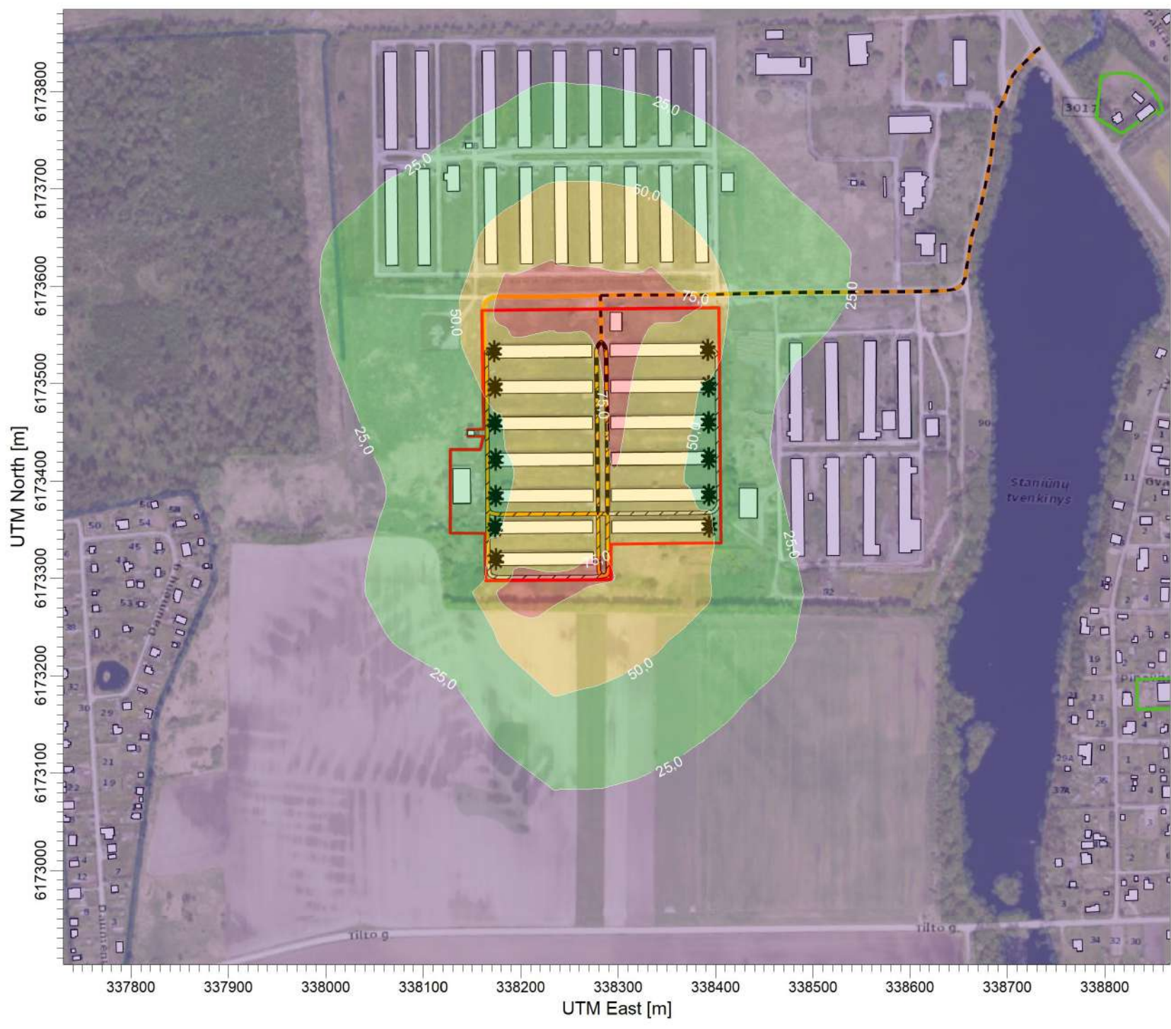
PLOT FILE OF 98.50TH PERCENTILE 1-HR VALUES FOR SOURCE GROUP: ALL Max: 90,3 [ug/m^3] at (338183,03, 6173585,10)
