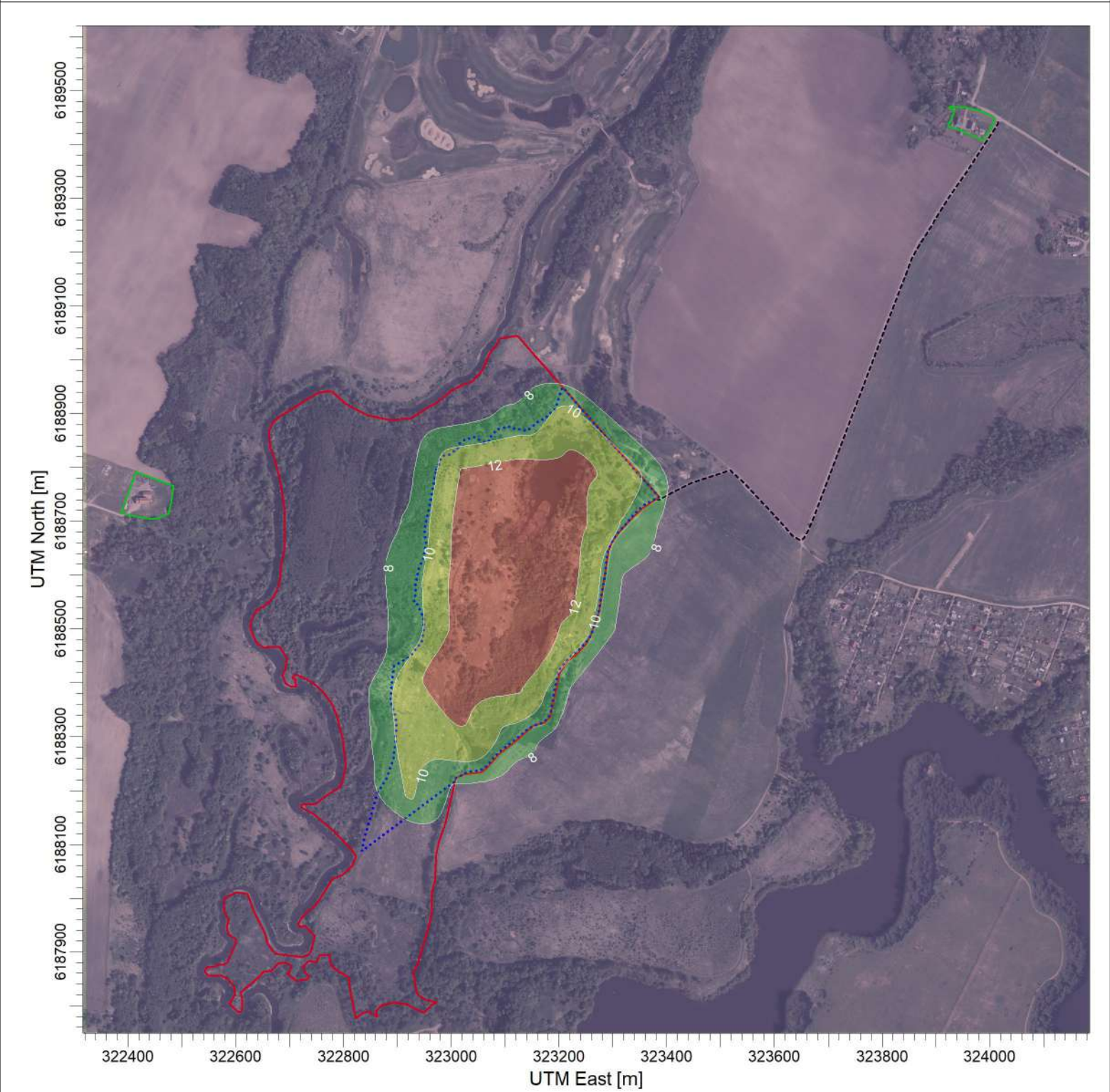
PLOT FILE OF ANNUAL VALUES AVERAGED ACROSS 5 YEARS FOR SOURCE GROUP: ALL Max: 13,5 [ug/m^3] at (323122,49, 6188691,70) ug/m^3
