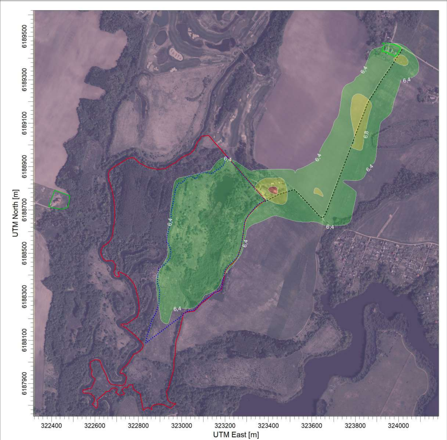
PLOT FILE OF ANNUAL VALUES AVERAGED ACROSS 5 YEARS FOR SOURCE GROUP: ALL Max: 7,4 [ \mu\text{g}/\text{m}^3 ] at (323422,49, 6188791,70) ug/m^3
